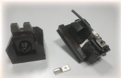
For tubular terminals
