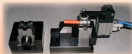
For battery terminals with integrated clamping
