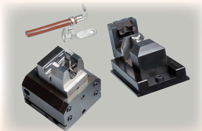
For terminals with crimping bending
