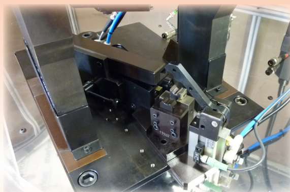
Band tool mounted in SEREC press
